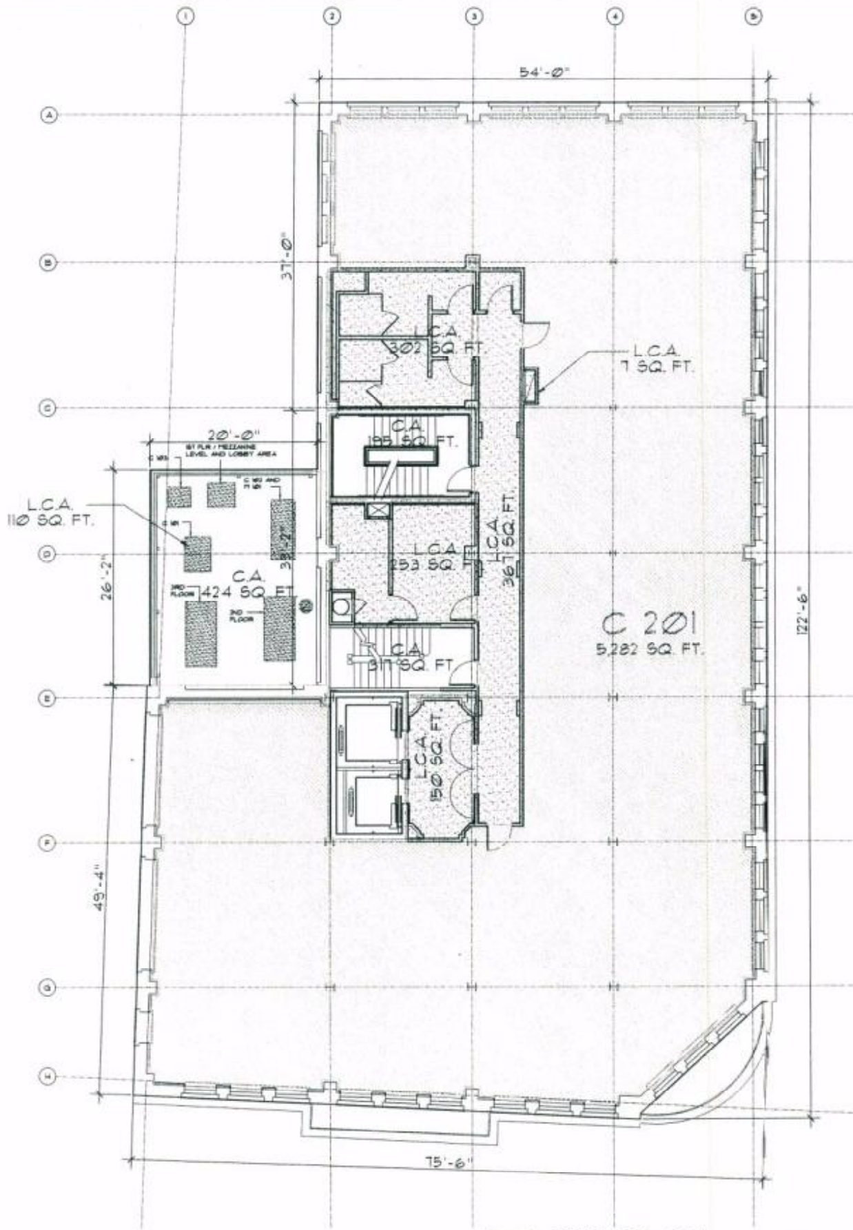
SECOND LEVEL FLOOR PLAN SCALE: 1/16" = 1'-0"
